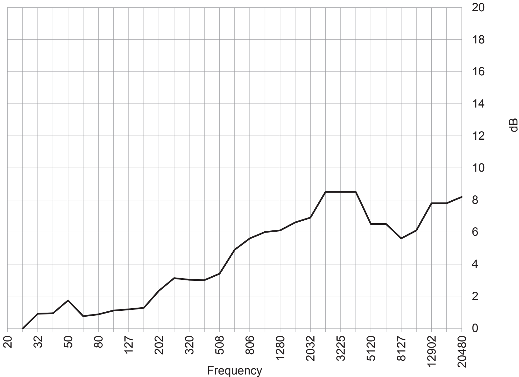
Directivity Index
